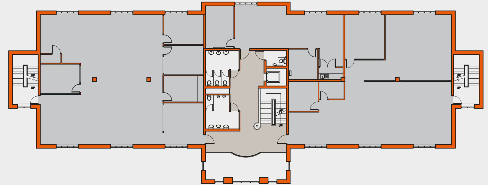
Third Floor:
